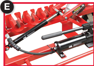
Hydraulic assisted boom lift/ one person setup • Set-up in 2 minutes with 1 person • Designed for optimal safety • Adjust boom to any angle
